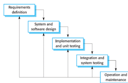
Gambar 3. Model Waterfall Menurut Ian Sommerville (2009) (Sumber: Ian Sommerville. 2009. Software Engineering - 9th ed)
