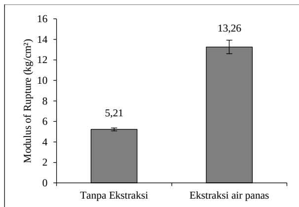
Gambar 6. Histogram Modulus of Rupture papan semen
