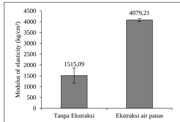
Gambar 5. Histogram Modulus of Elasticity papan semen
