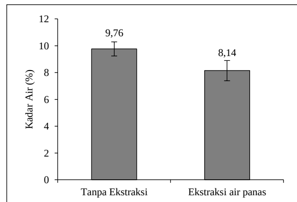
Gambar 1. Histogram kadar air papan semen
