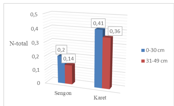
Gambar 5. Nilai N-total (%)
