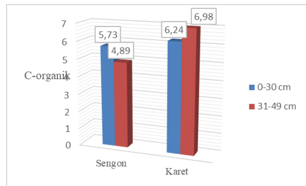
Gambar 4. Nilai C-organik (%)
