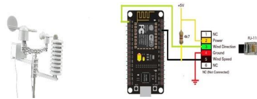
Gambar 10. Wind Speed dan Wind Direction
