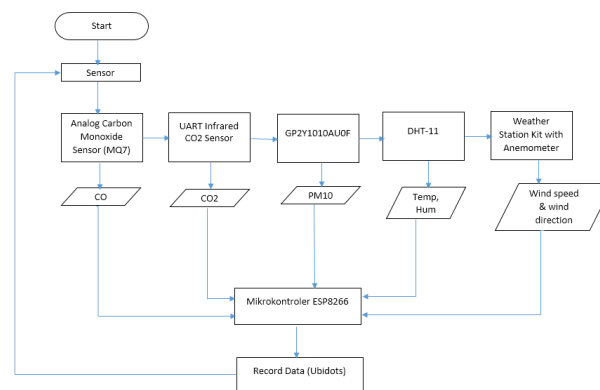
Gambar 12. Diagram alur kerja sensor
