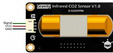
Gambar 8. Analog Infrared CO2
