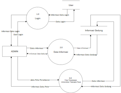
Gambar 4.2 DFD Level 2
